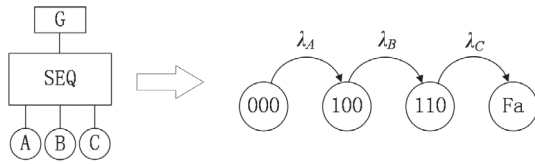
FIGURE 5 SEQ conversion to Markov model
