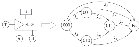
FIGURE 6 FDEP conversion to Markov model
