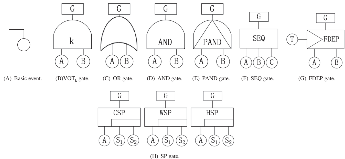
FIGURE 3 Node types in (A)–(D) static and (all) dynamic fault trees
