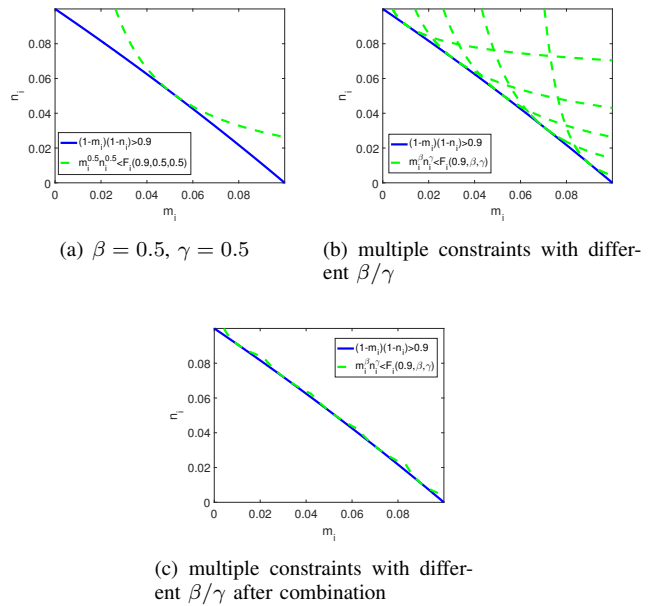
Fig. 1. Comparison between constraint (20) after linear approximation and nonlinear constraint (16) when \alpha = 0.9 .
